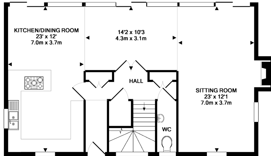
GROUND FLOOR APPROX. FLOOR AREA 893 SQ.FT. (82.9 SQ.M.)
